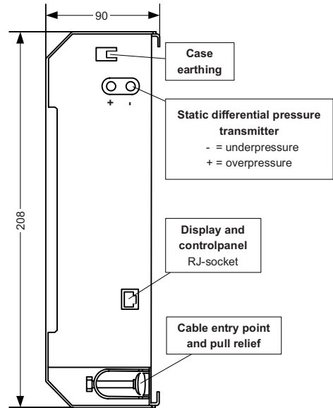
Case FM500: Side view
