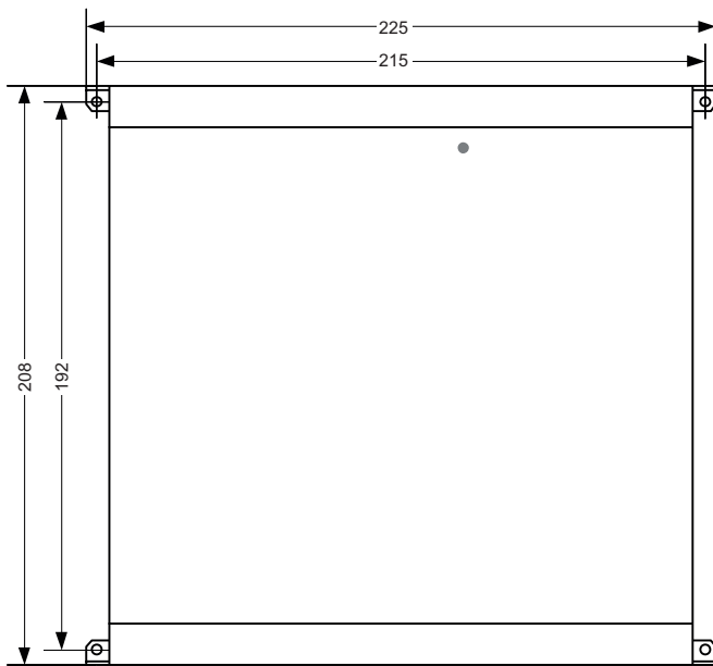
Case FM500: Top view
